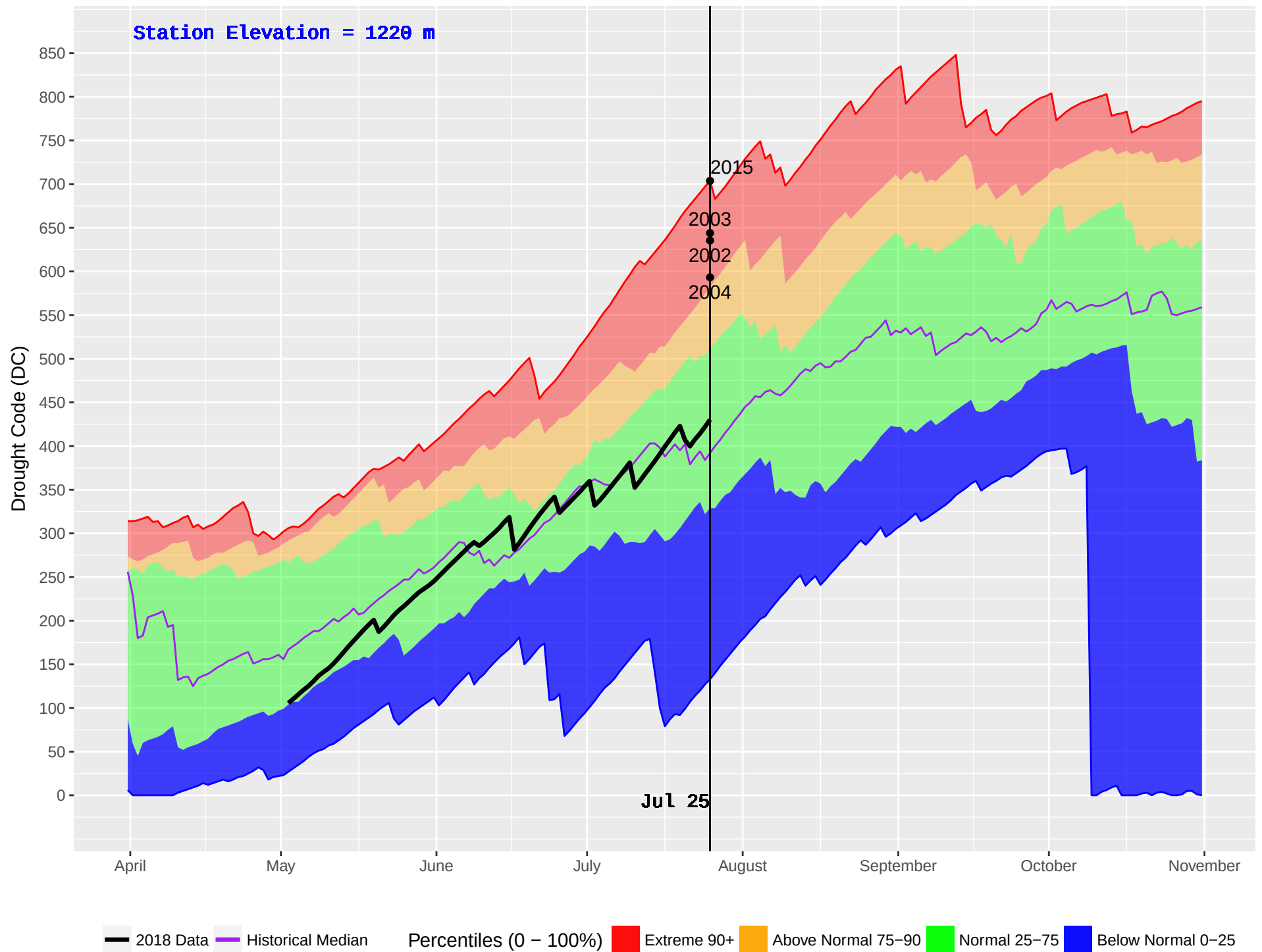
NEMIAH (216) : Historical (1982–2016) and Current (2018) Noon Drought Code (DC)
